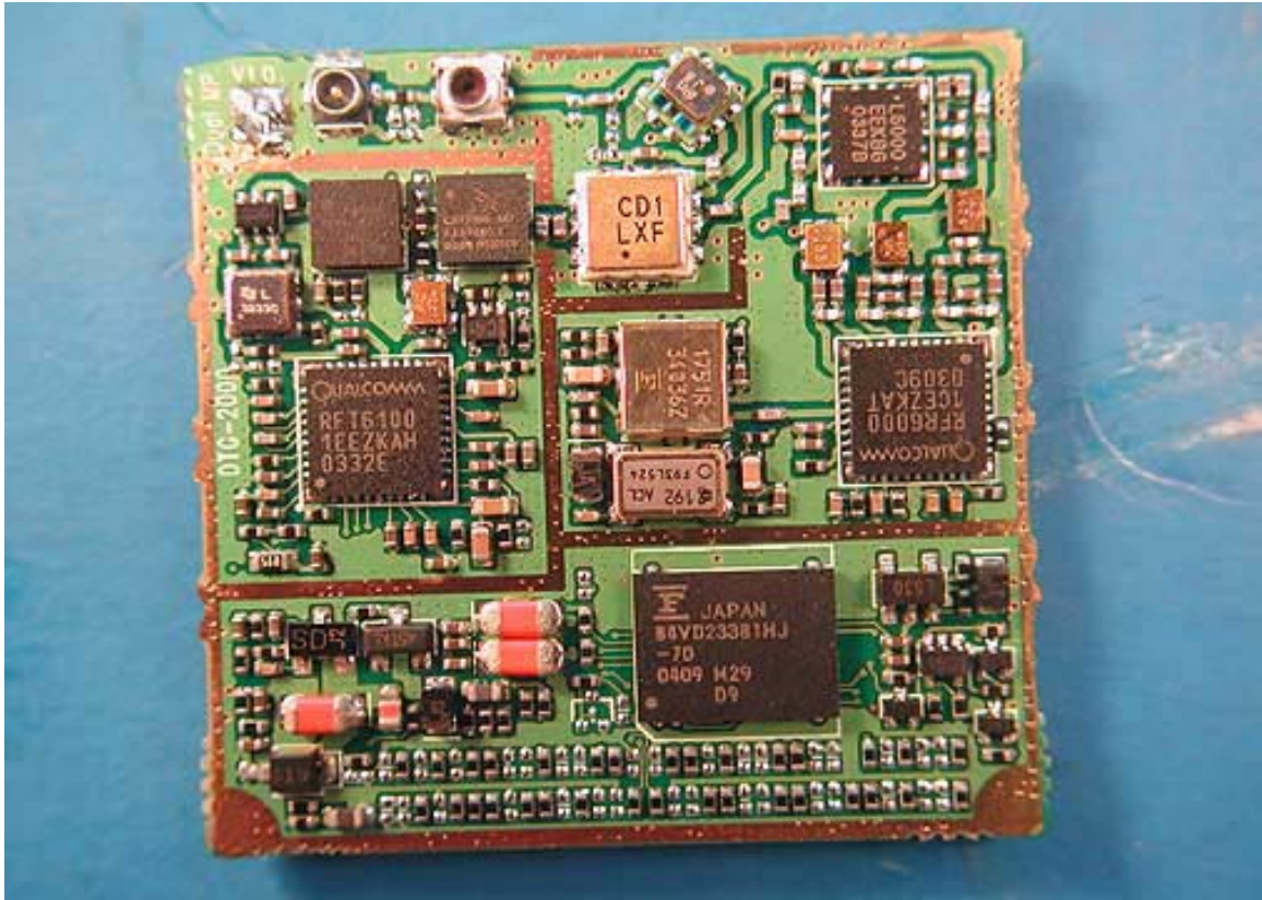
RF PCB Front
