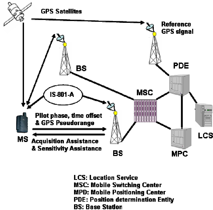
Figure 1.2 : GPSOne system architecture in control plan
