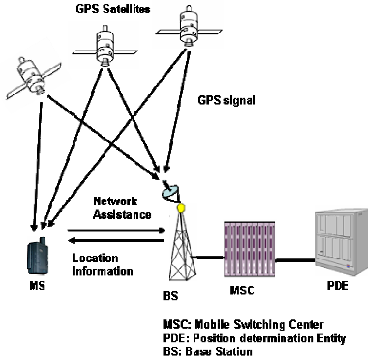
A-GPS wireless network infrastructure
