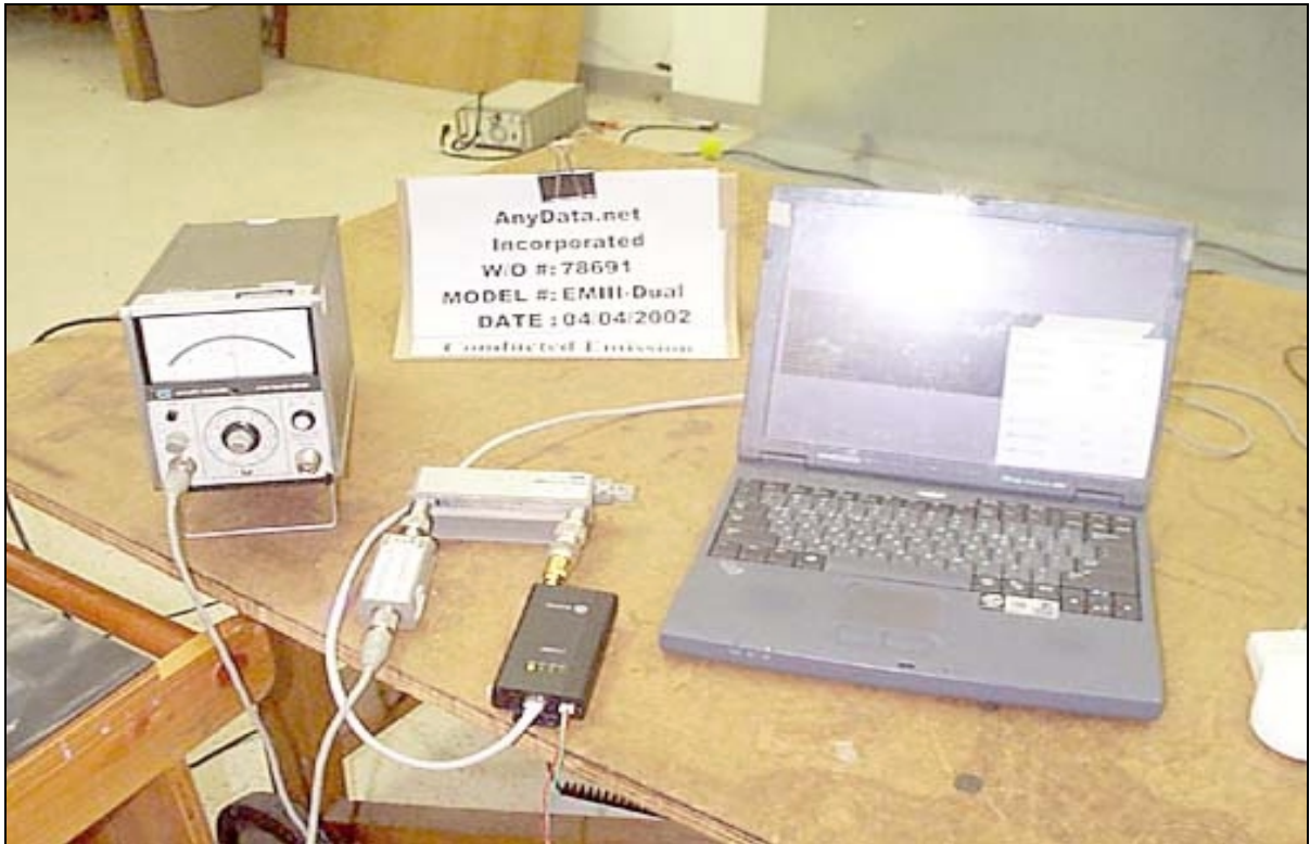
Carrier Output Power Test Setup
