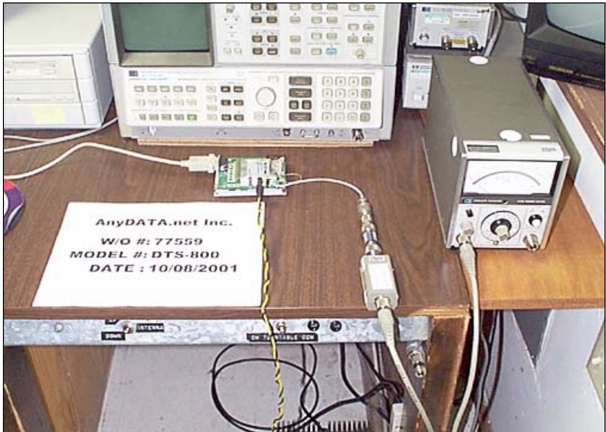
Setup for Direct Connect Testing
