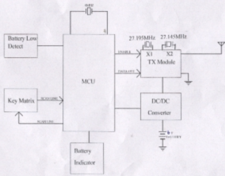
RF-711 BLOCK DIAGRAM
