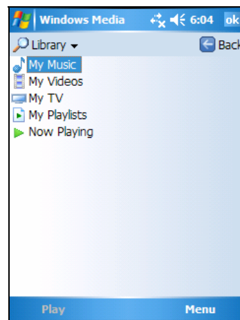
Library Screen
