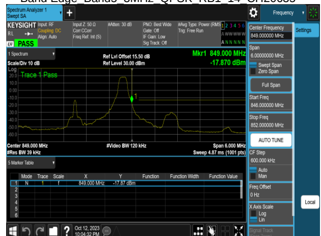
Band Edge Band5 3MHz QPSK RB1 14 CH20635
