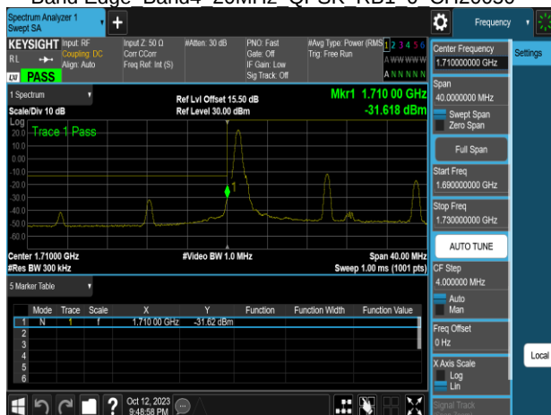
Band Edge Band4 20MHz QPSK RB1 0 CH20050
