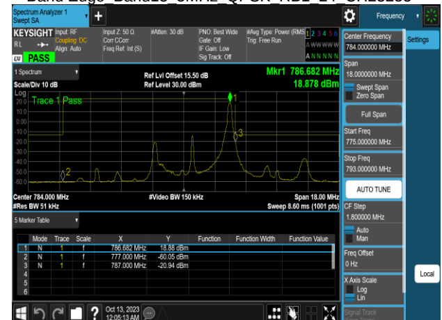
Band Edge Band13 5MHz QPSK RB1 24 CH23255
