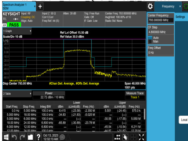
Emission Mask Band14 10MHz QPSK RB50 0 CH23330
