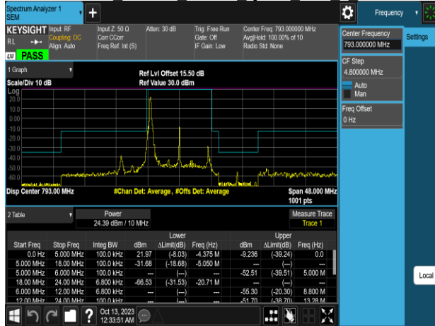
Emission Mask Band14 10MHz QPSK RB1 49 CH23330
