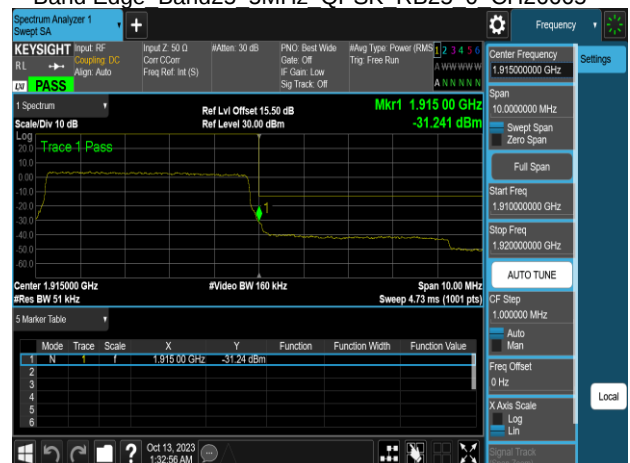
Band Edge Band25 5MHz QPSK RB25 0 CH26665
