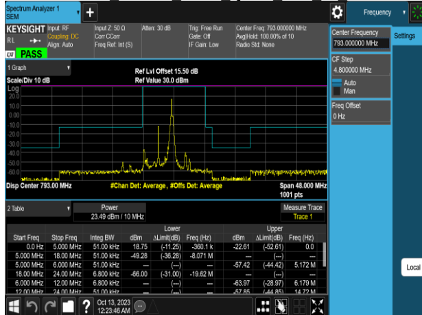
Emission Mask Band14 5MHz QPSK RB1 24 CH23330
