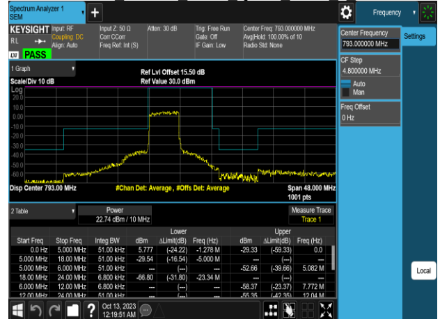
Emission Mask Band14 5MHz QPSK RB25 0 CH23330
