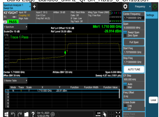
Band Edge Band66 3MHz QPSK RB15 0 CH131987
