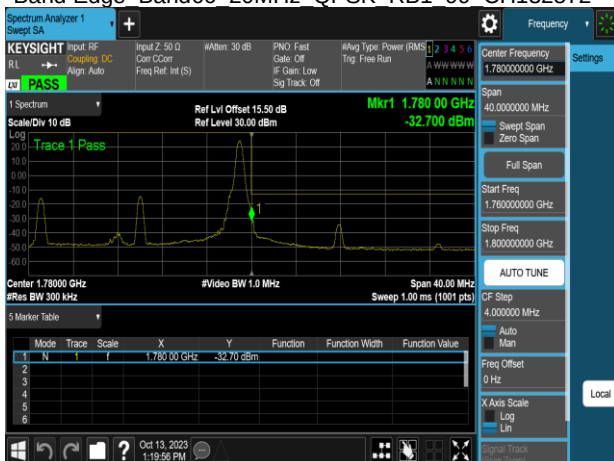
Band Edge Band66 20MHz QPSK RB1 99 CH132572
