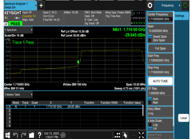
Band Edge Band66 5MHz QPSK RB25 0 CH132647
