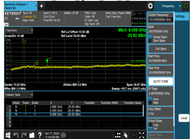
Band41 5MHz QPSK RB1 0 CH41565
