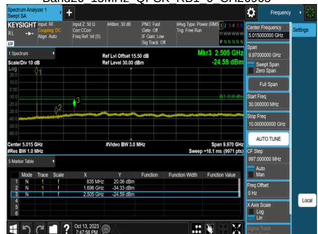
Band26 15MHz QPSK RB1 0 CH26965
