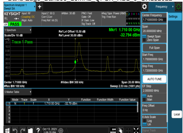
Band Edge Band66 10MHz QPSK RB1 0 CH132022
