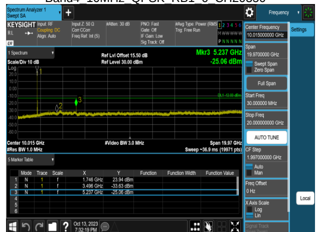
Band4 10MHz QPSK RB1 0 CH20350
