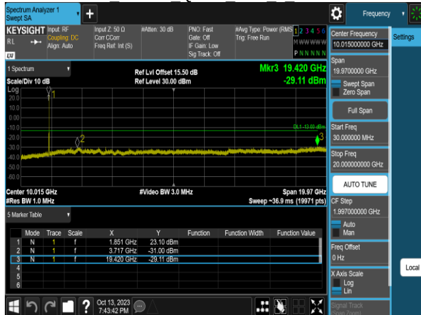
Band25 20MHz QPSK RB1 0 CH26365
