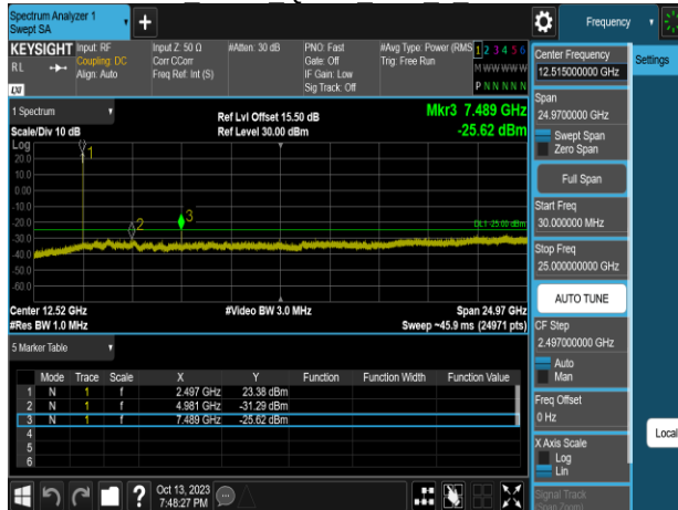
Band41 5MHz QPSK RB1 0 CH39715
