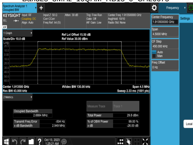
Band25 3MHz 16QAM RB15 0 CH26675
