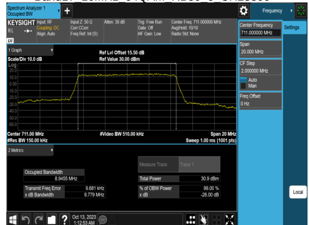
Band17 10MHz 64QAM RB50 0 CH23800
