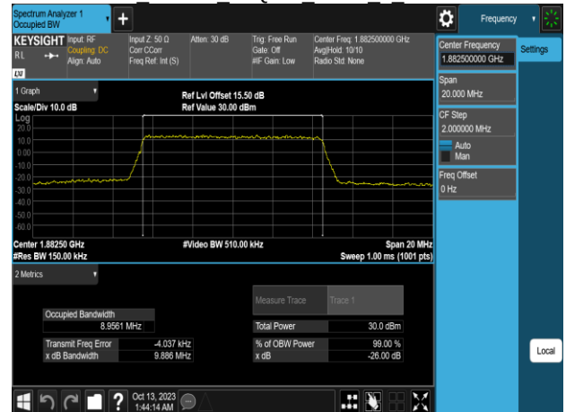
Band25 10MHz 64QAM RB50 0 CH26640
