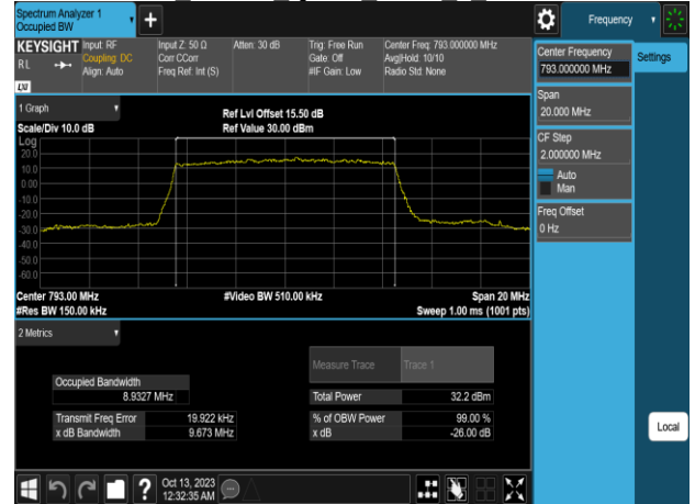
Band14 10MHz 16QAM RB50 0 CH23330
