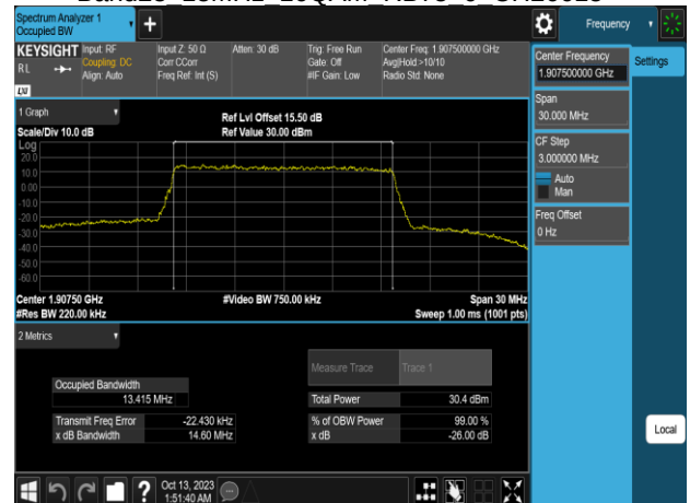
Band25 15MHz 16QAM RB75 0 CH26615
