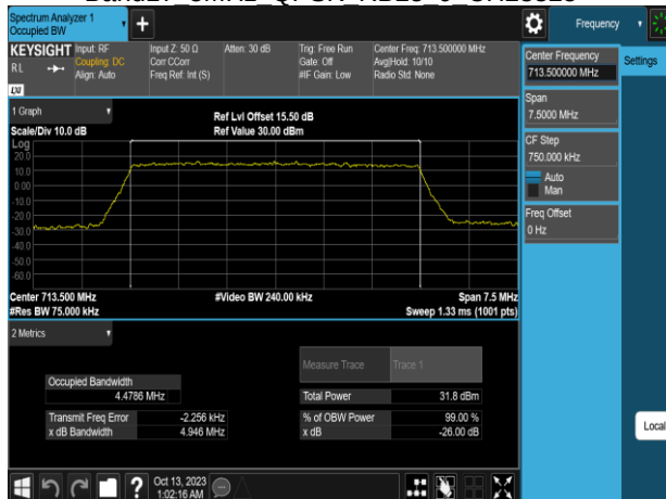
Band17 5MHz QPSK RB25 0 CH23825
