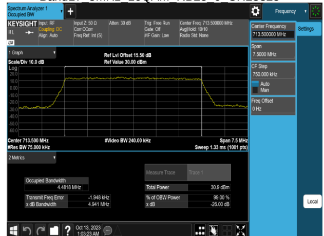
Band17 5MHz 16QAM RB25 0 CH23825
