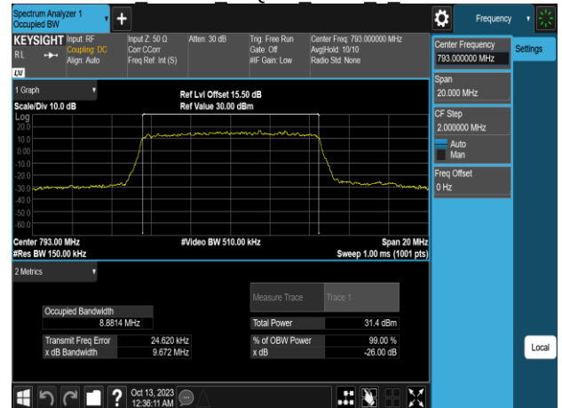
Band14 10MHz 64QAM RB50 0 CH23330
