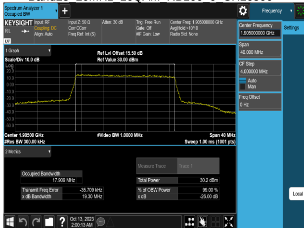
Band25 20MHz 16QAM RB100 0 CH26590
