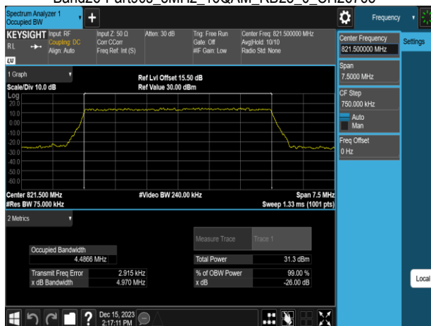
Band26-Part90s_5MHz_16QAM_RB25_0_CH26765
