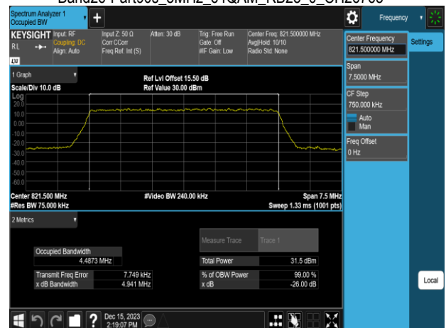
Band26-Part90s_5MHz_64QAM_RB25_0_CH26765
