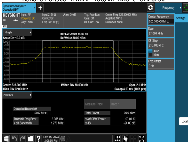
Band26-Part90s_1.4MHz_16QAM_RB6_0_CH26783
