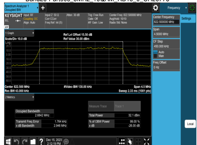
Band26-Part90s_3MHz_16QAM_RB15_0_CH26775
