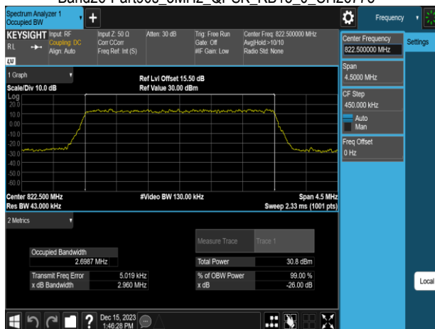
Band26-Part90s_3MHz_QPSK_RB15_0_CH26775
