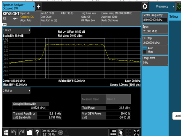
Band26-Part90s_10MHz_64QAM_RB50_0_CH26740
