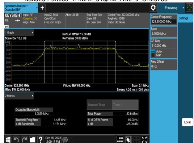
Band26-Part90s_1.4MHz_64QAM_RB6_0_CH26783
