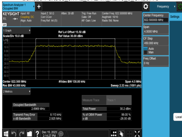
Band26-Part90s_3MHz_64QAM_RB15_0_CH26775
