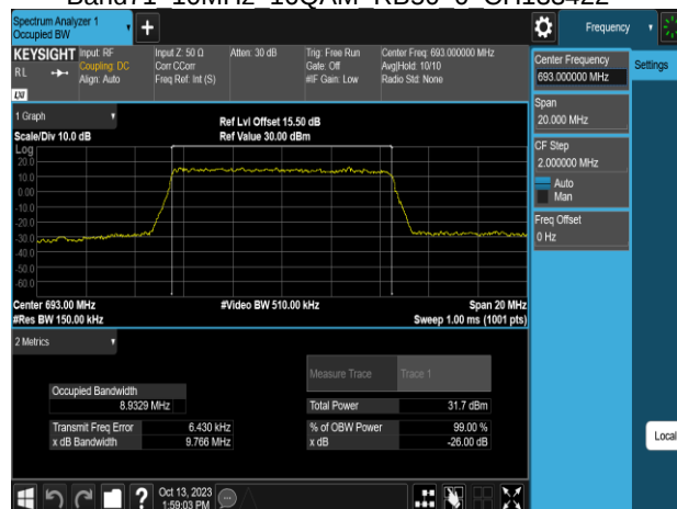
Band71 10MHz 16QAM RB50 0 CH133422
