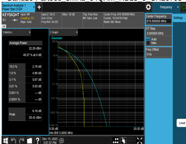
Band26-Part90s 3MHz 64QAM RB15 0 CH26705
