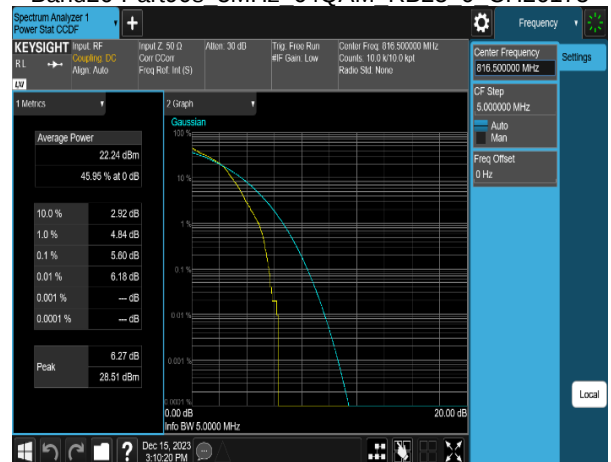
Band26-Part90s 5MHz 64QAM RB25 0 CH26175
