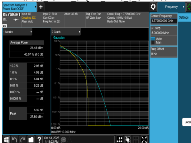
Band66 15MHz 64QAM RB75 0 CH132597
