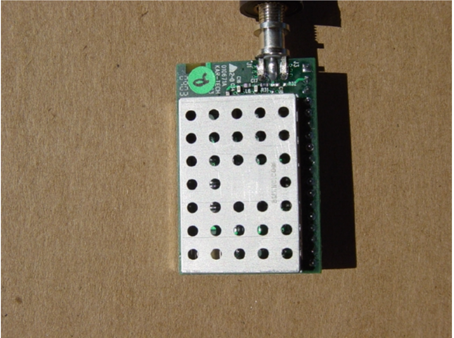
Closeup of EUT with shield
