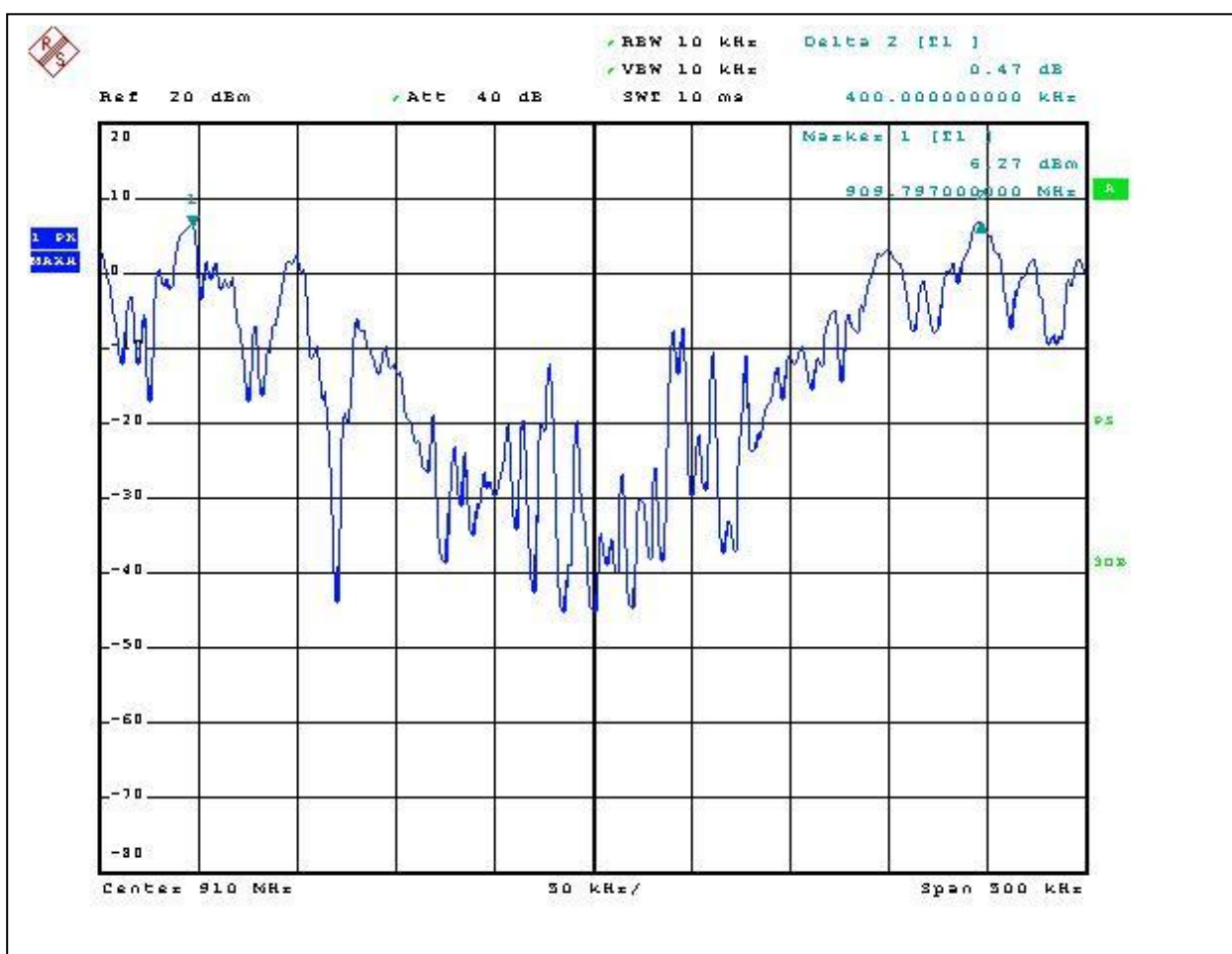
Graph # 3-2-1 Hopping Channel Carrier Frequency Separation
