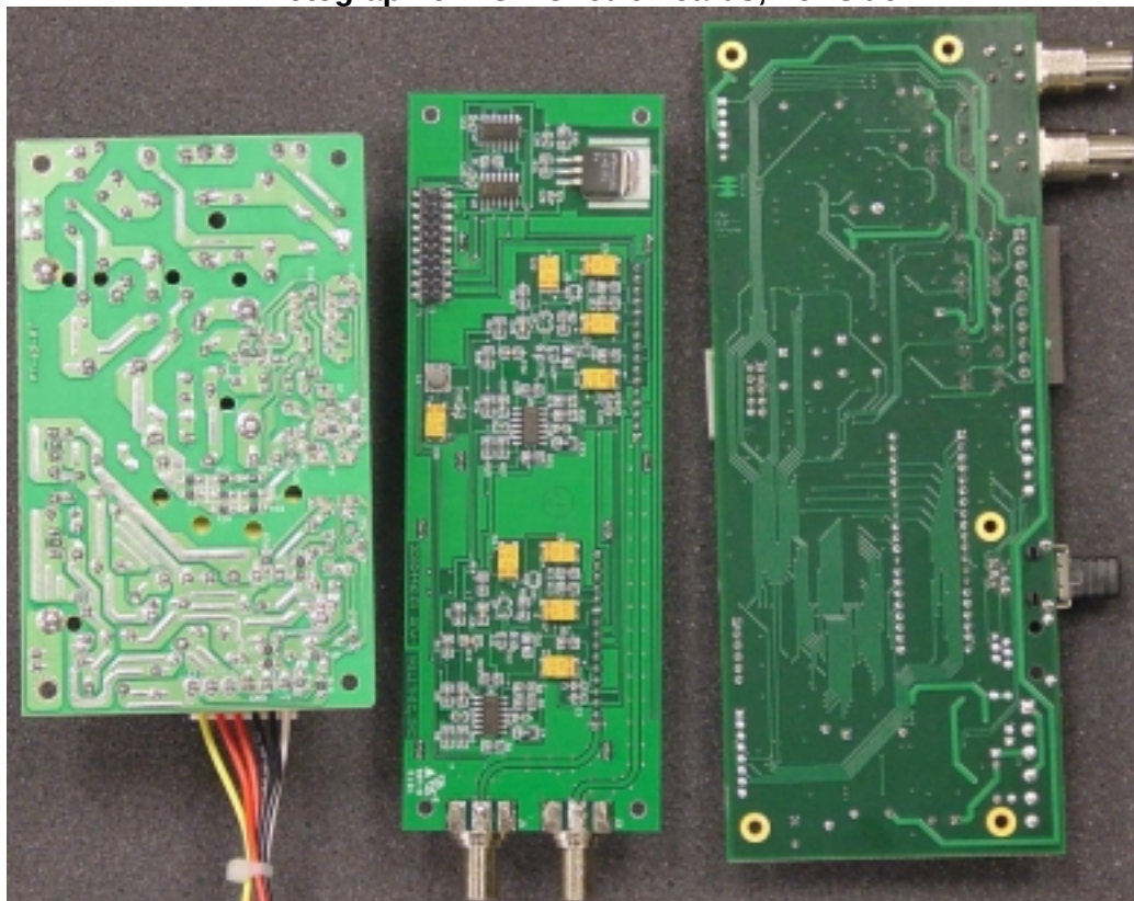
Photograph of EUT Circuit Boards; Foil side
