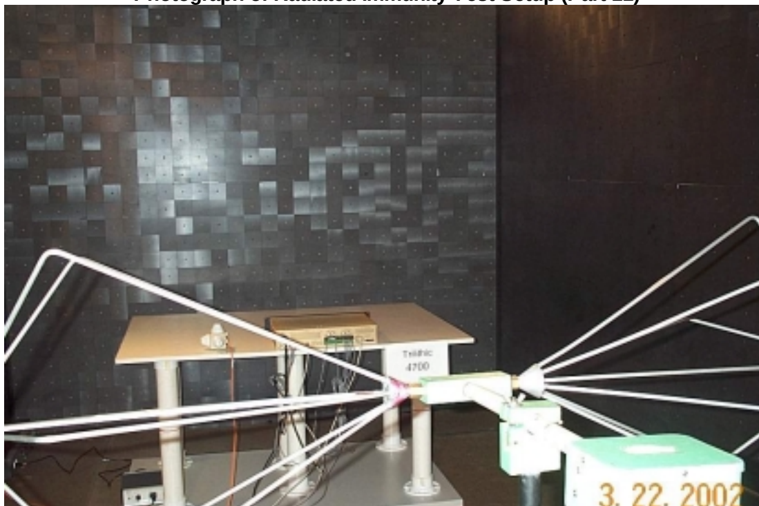
Photograph of Radiated Immunity Test Setup (Part 11)
