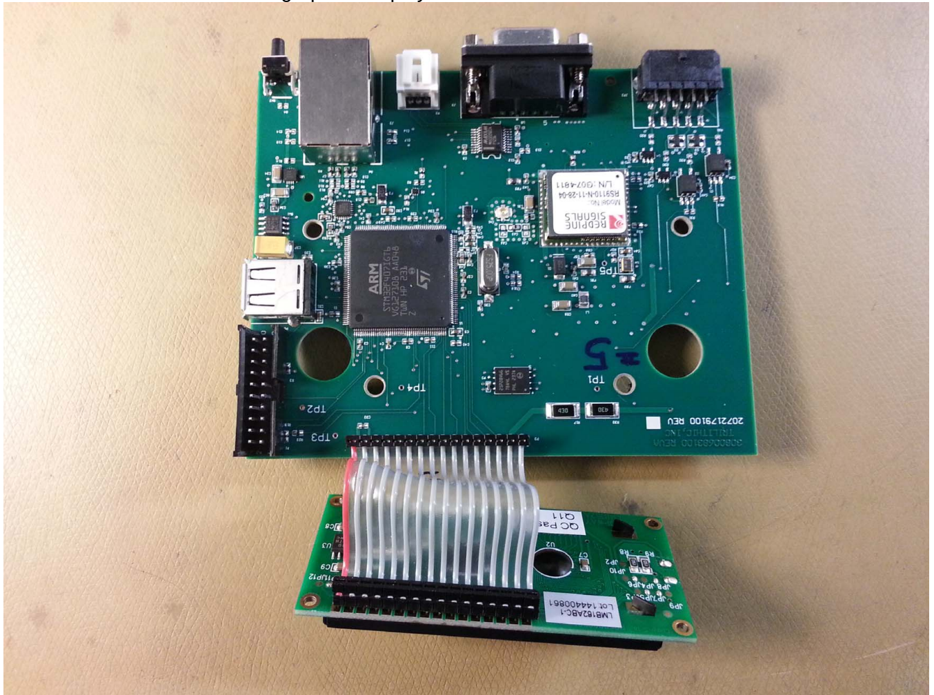
Photograph of Display module installed on Main PCB
