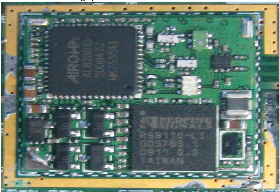
Photograph of Wifi Module with shield removed
