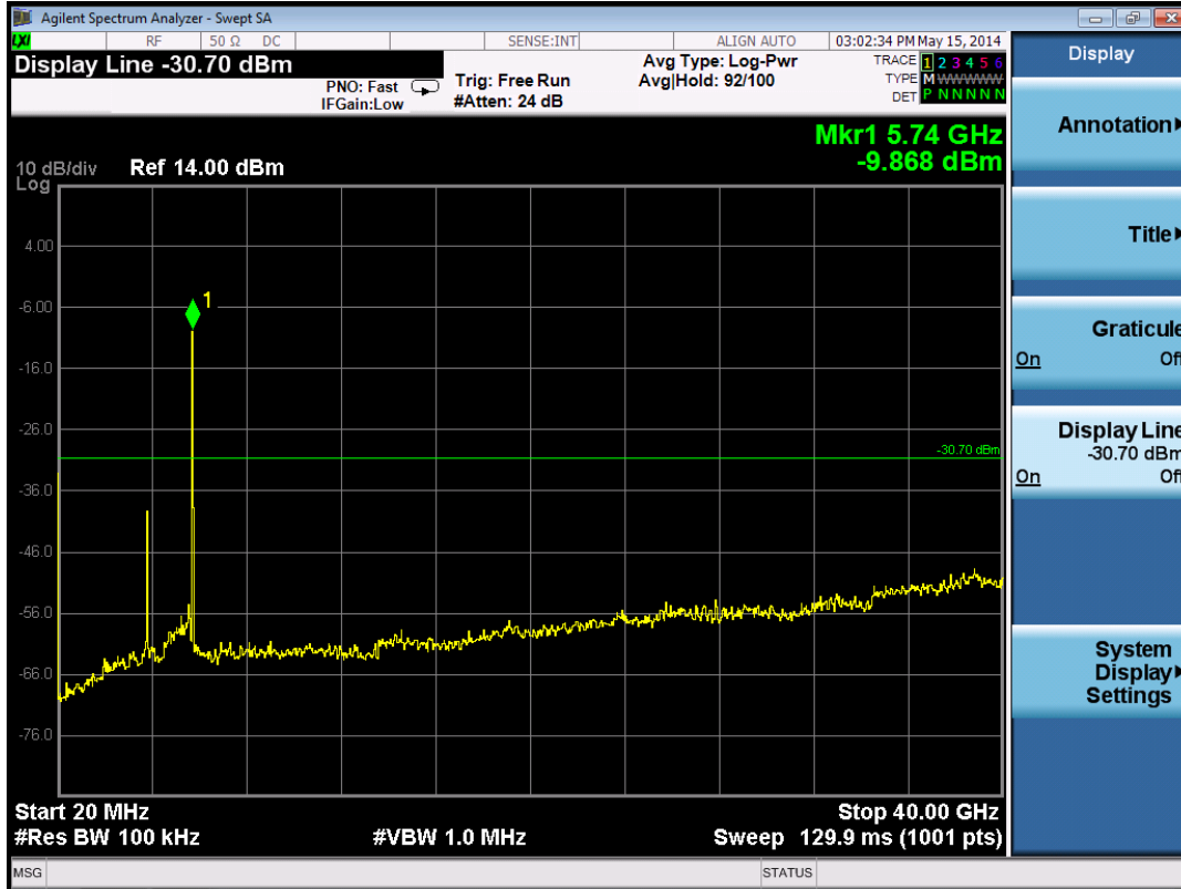
802.11g Channel 149
