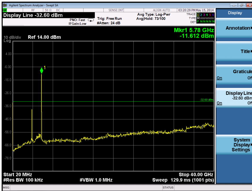
802.11N Channel 157
