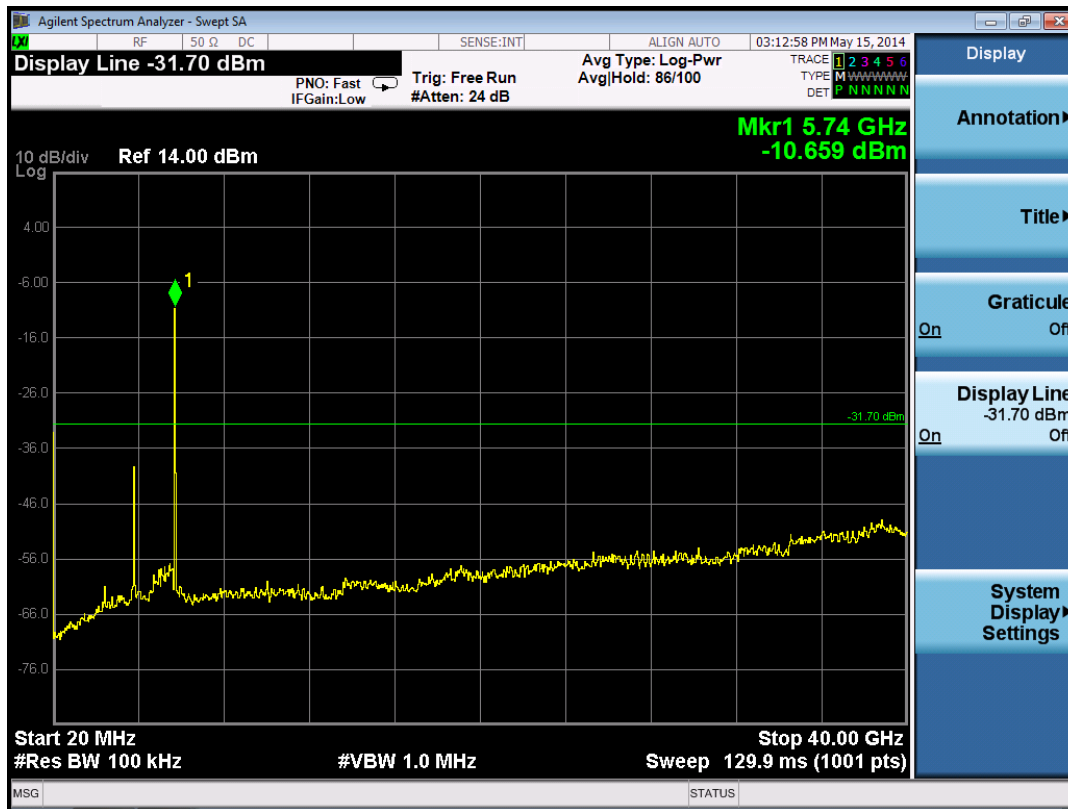
802.11N Channel 149
