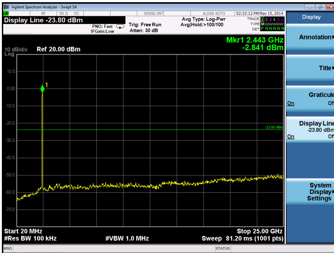
802.11N Channel 6
