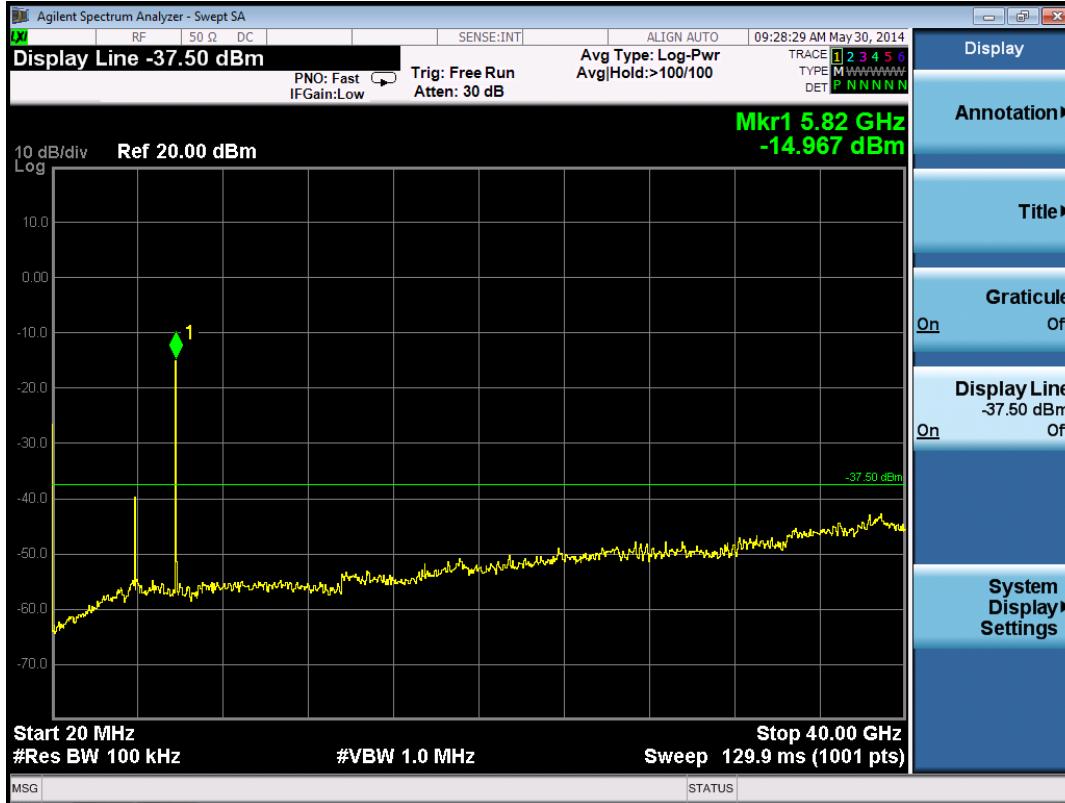
802.11N Channel 165
