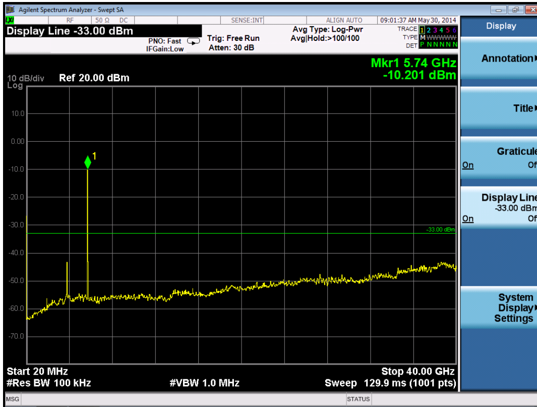
802.11A Channel 149
