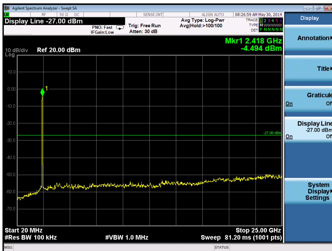
802.11N Channel 1
