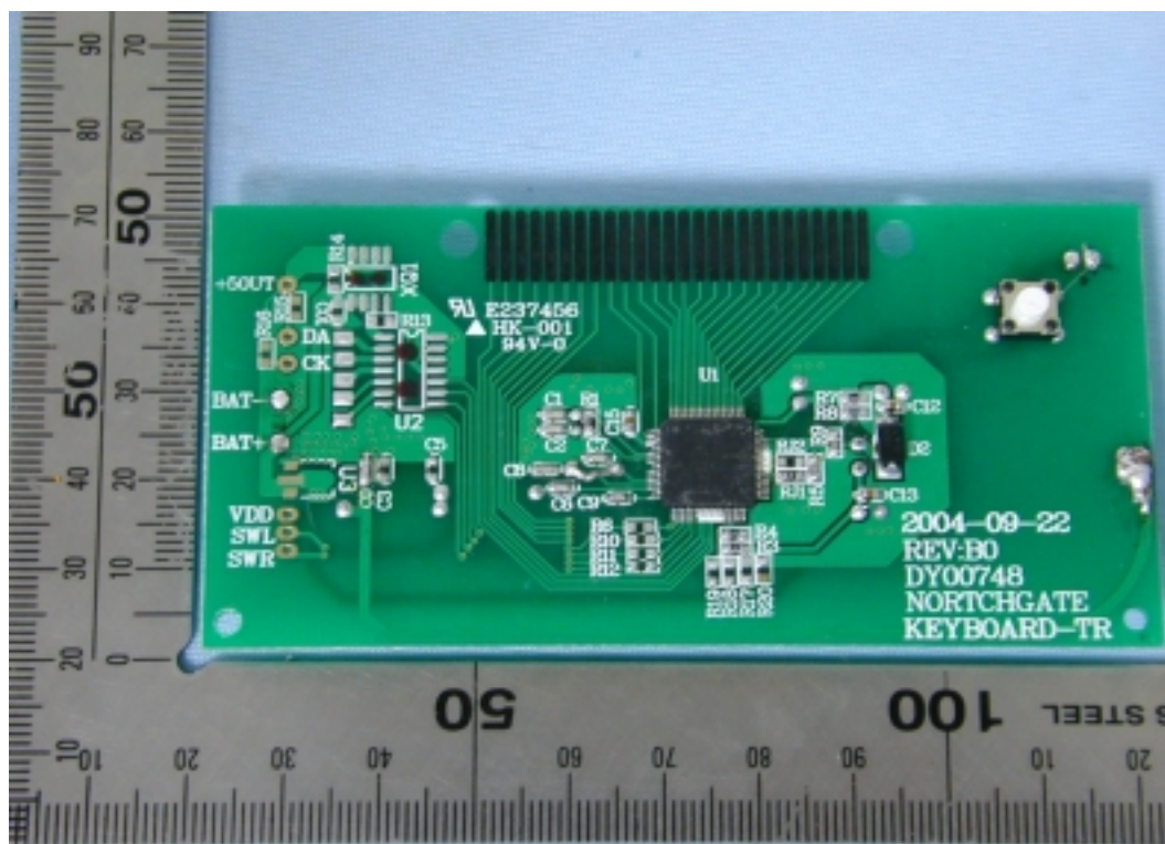
Full View of Component
