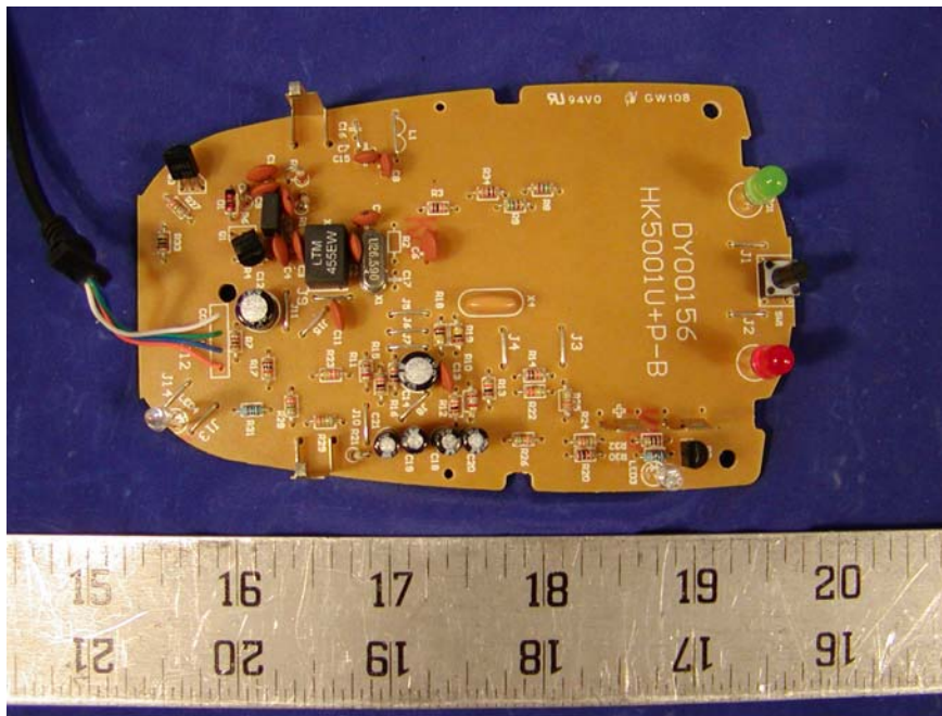
Receiver Main Board - Solder View
