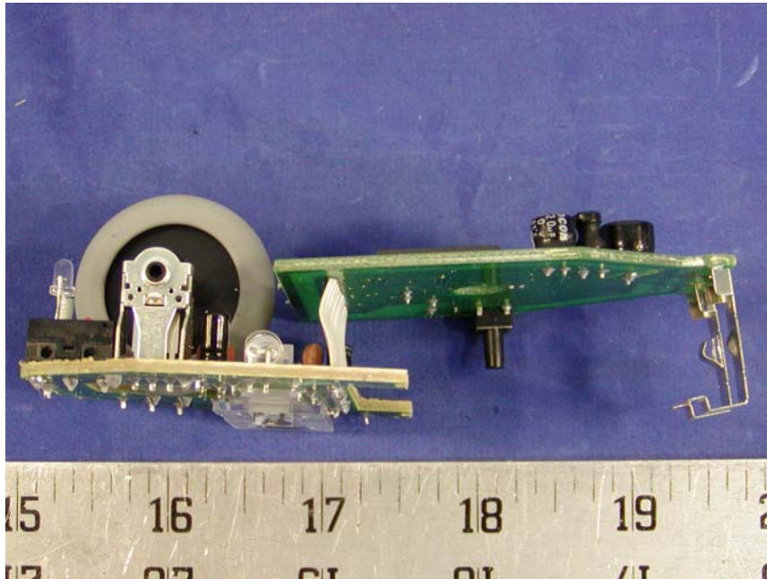
Transmitter Main Board – Side View
