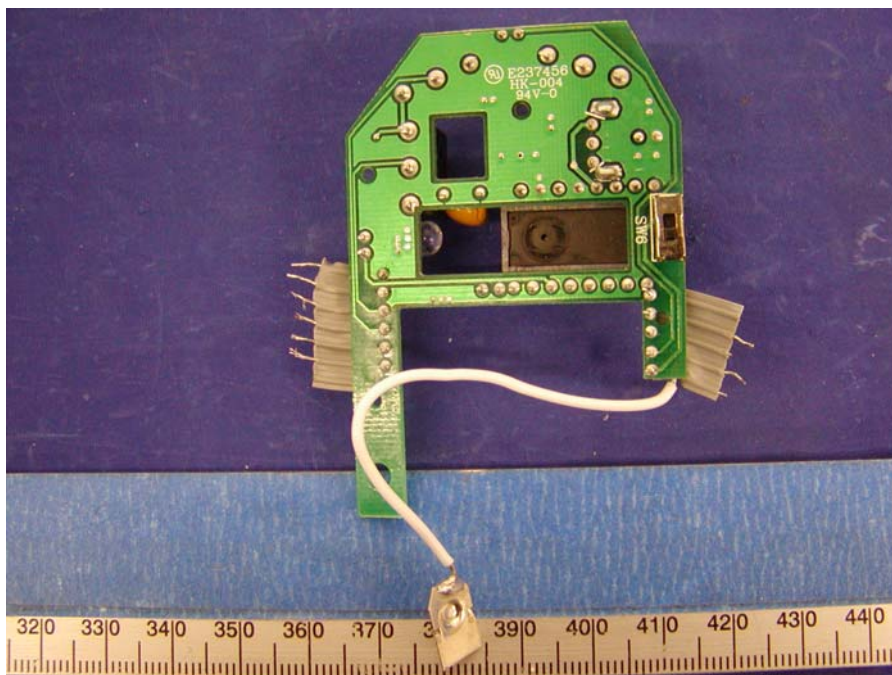
EUT – Solder View I
