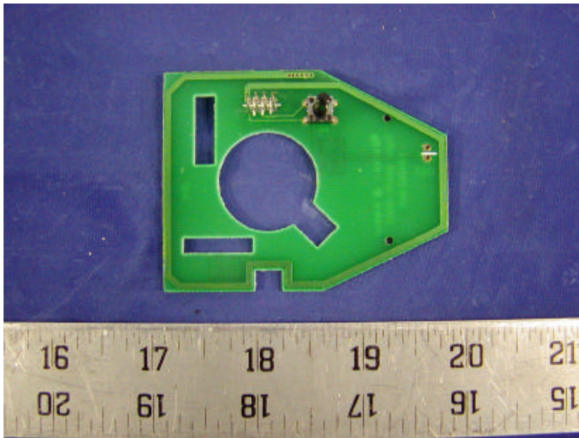
Antenna Board – Component View
