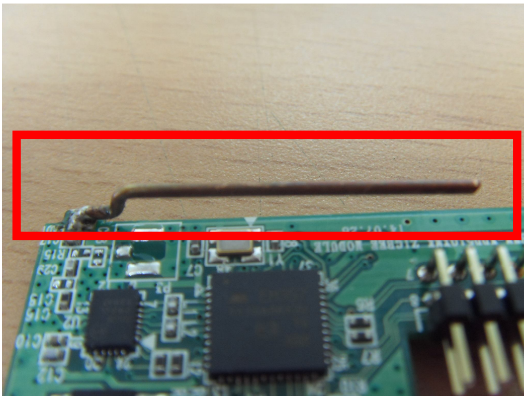
Zigbee Antenna
