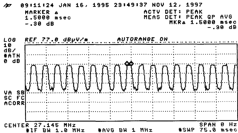
Figure C [Short Pulse]
