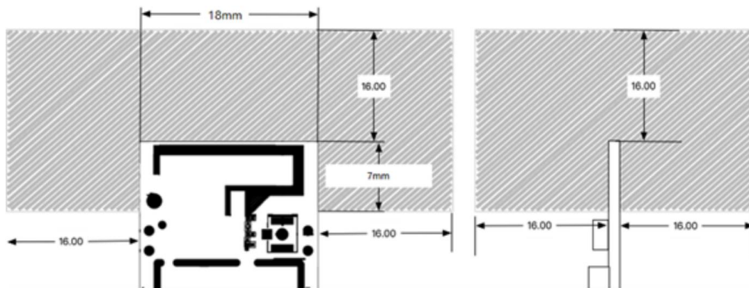
PCB Antenna Minimum Clearance (unit: mm)
