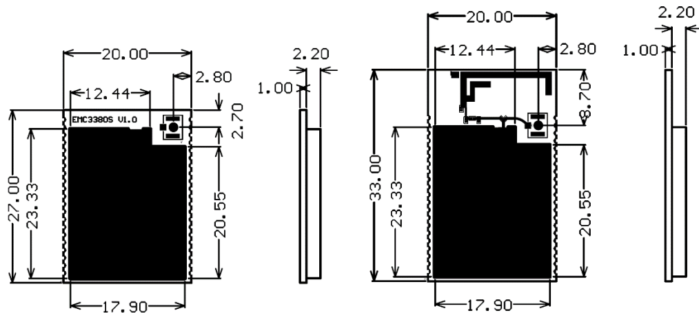
Figure 12 EMC3380-S, EMC3380-D dimension (unit: mm)
