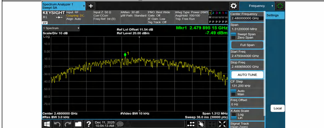
BLE_1M-Ant1-2480-PASS
