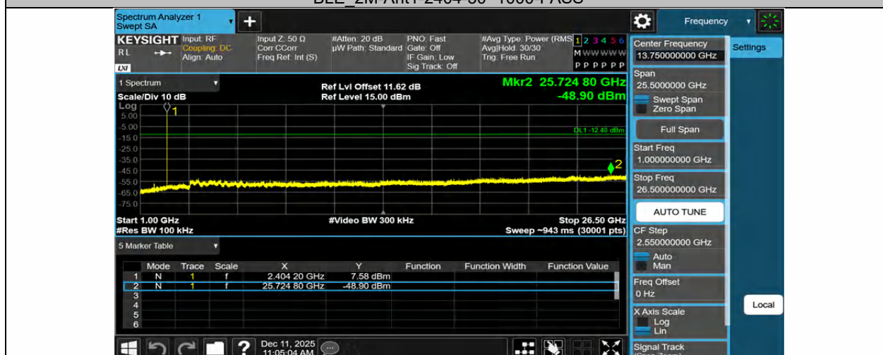
BLE_2M-Ant1-2404-1000~26500-PASS
