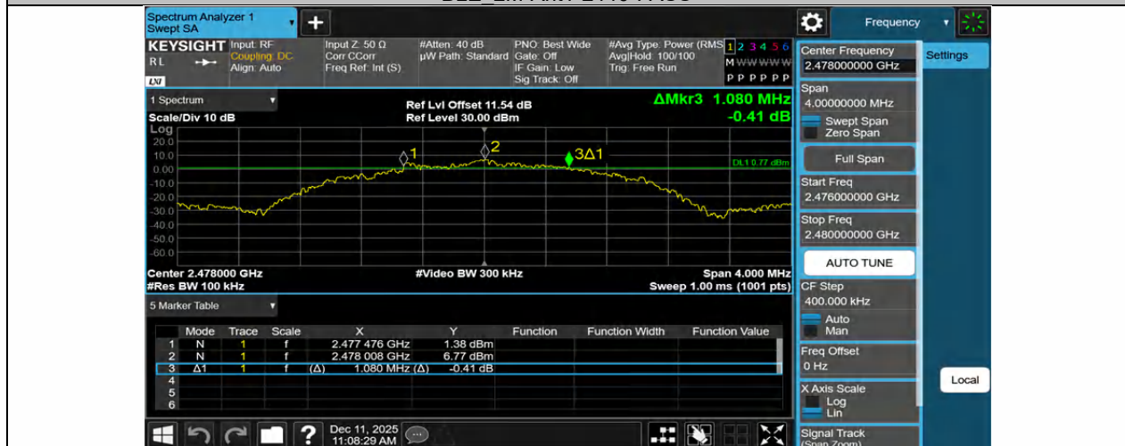
BLE_2M-Ant1-2478-PASS
