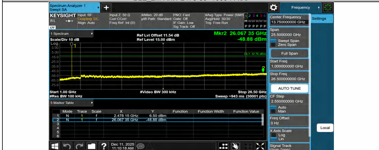
BLE_2M-Ant1-2478-1000~26500-PASS
