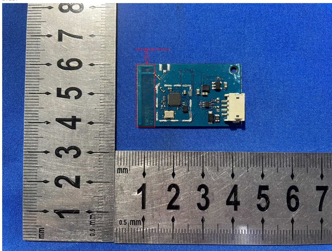
Photo 3: Internal View for 2.4G-WiFi/BLE Antenna
