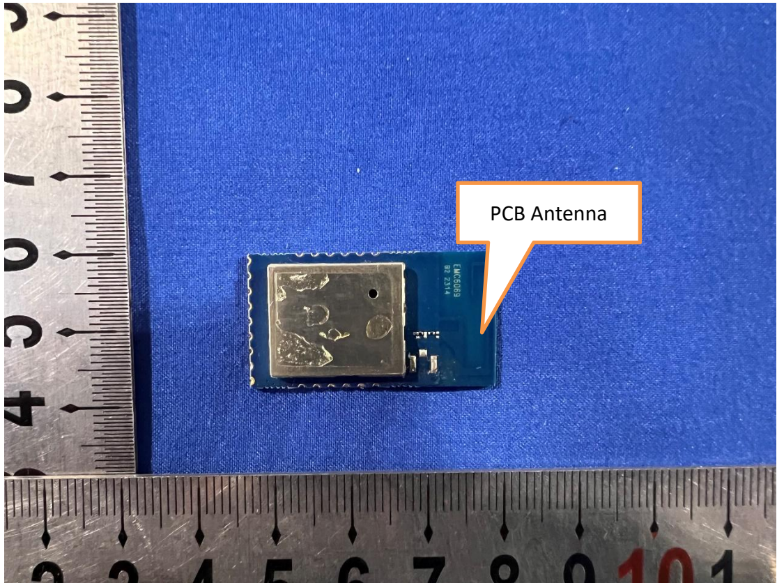
Photo 3: Antenna
