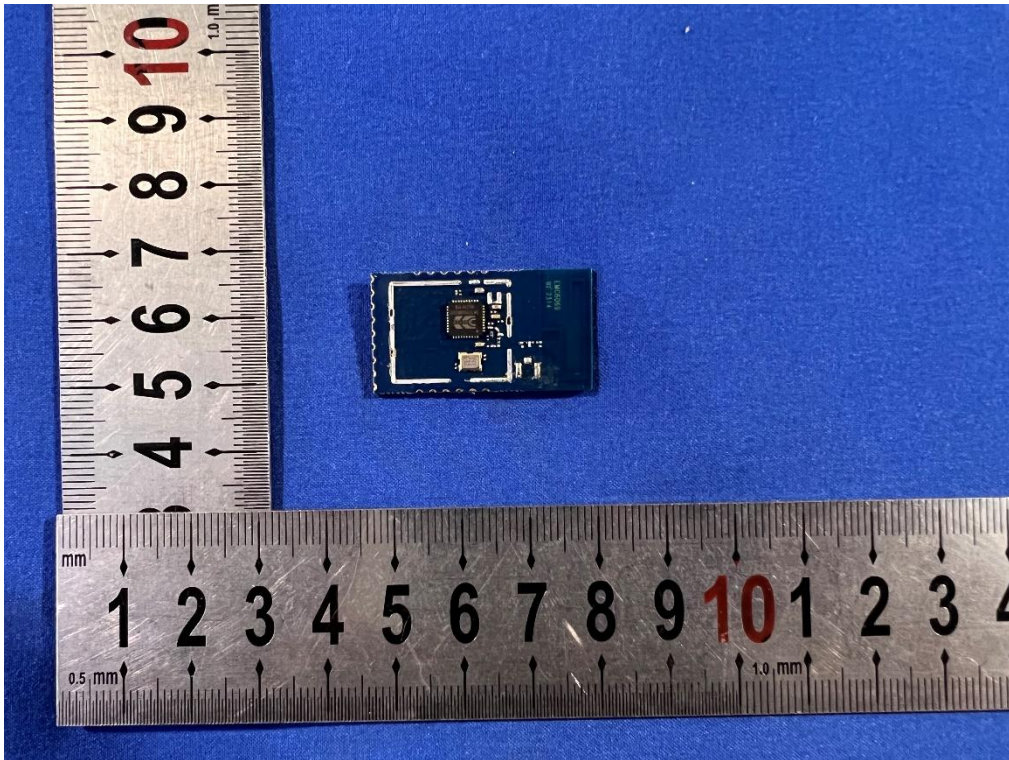
Photo 1:PCB view
