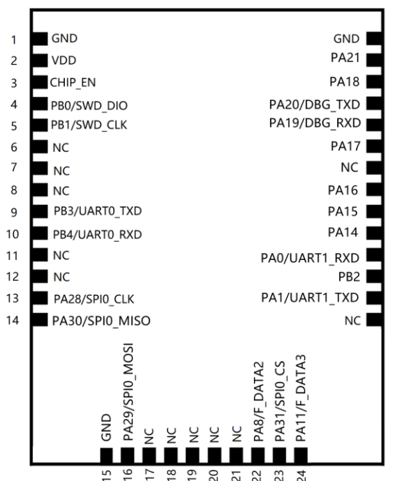
Figure 1 Pin Arrangement
