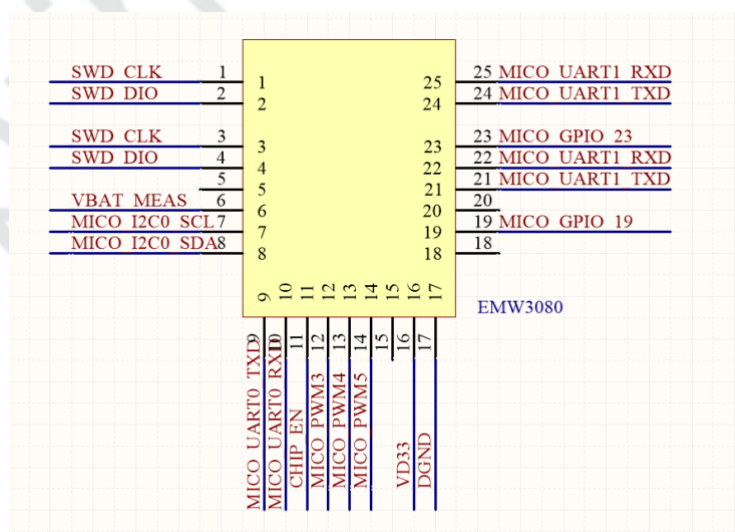
Figure 15 External Interface Circuit of EMW3080V2
