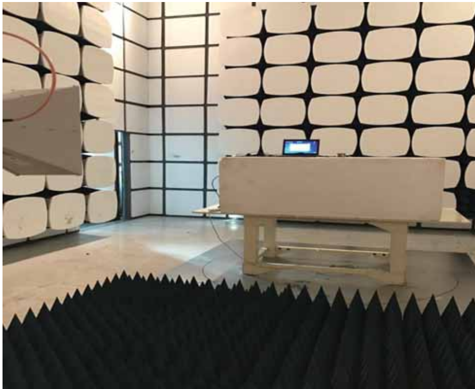
EUT with evaluation board
