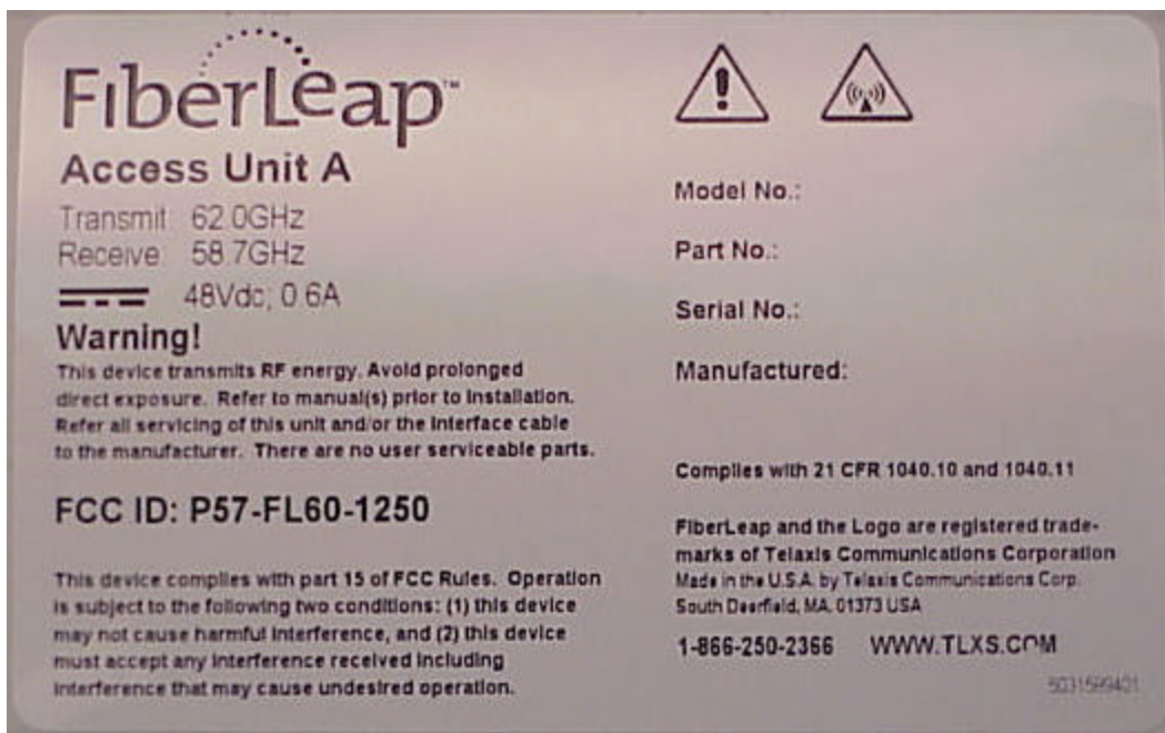
Photograph 1: EUT Label Access Unit A
