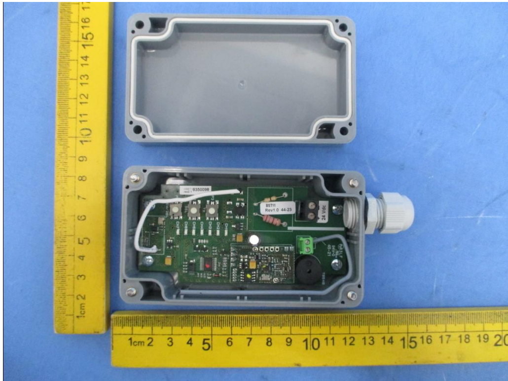
Internal Photo FCC ID: P59BST11 IC: 11242A-BST11
