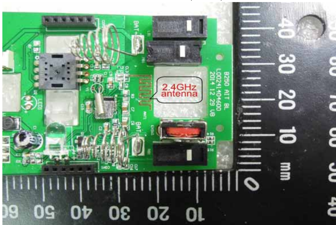
Antenna Location (B250 3B)
