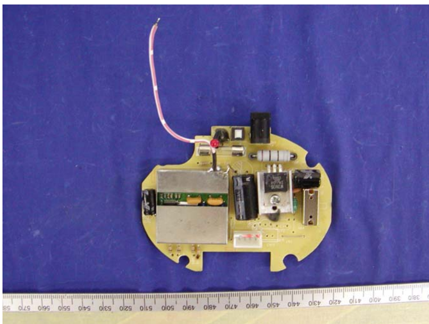
Transmitter – Main Board Component View
