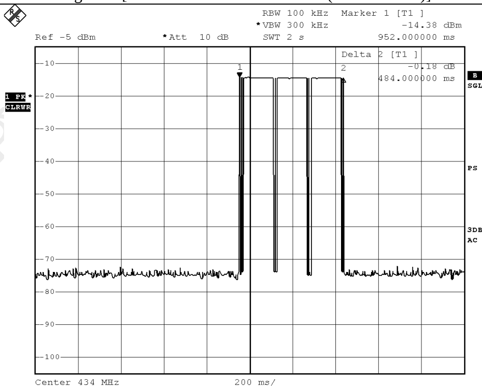
Figure C [Duration of each transmission ( =0.484\text{ s} < 1\text{ s} )]
