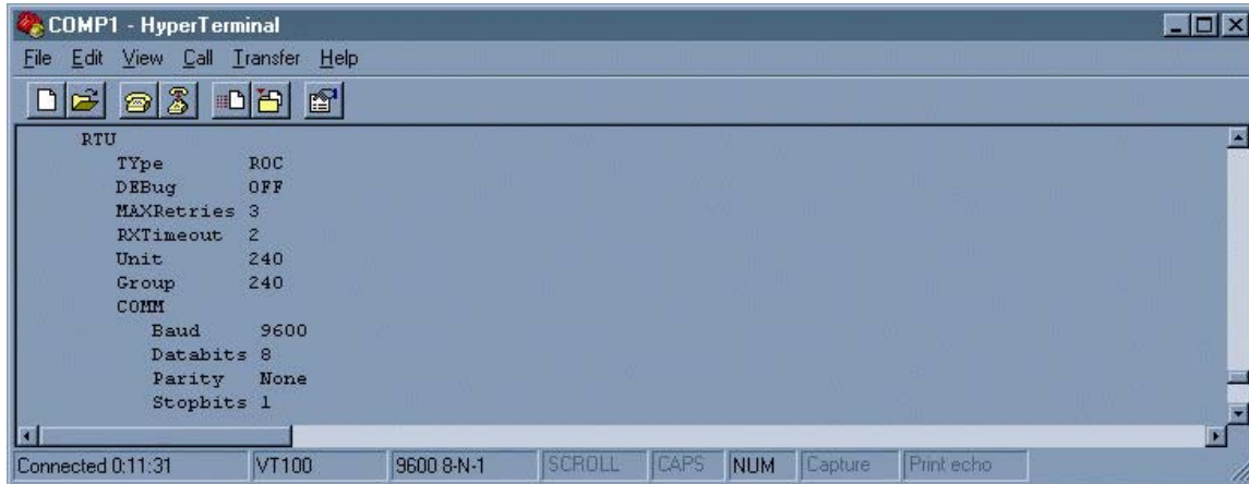
Figure 23: ROC Configuration
