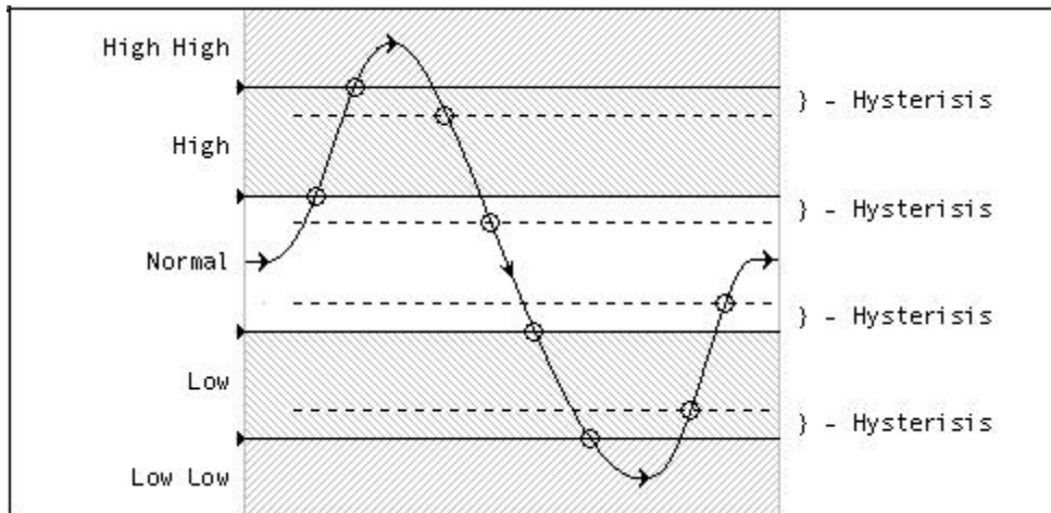
Figure 15: Alarm Hysterisis
