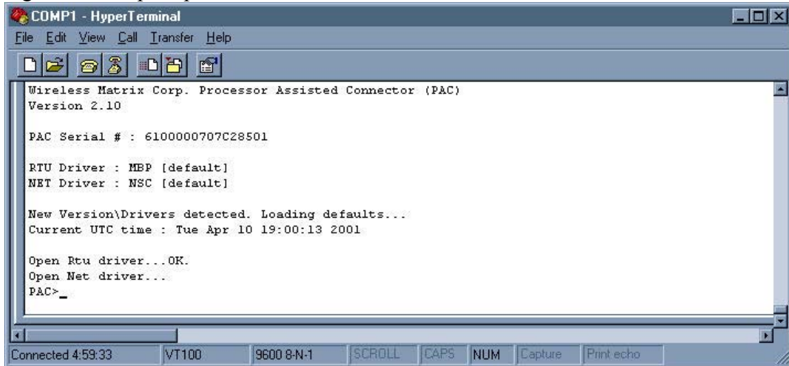
Figure 7: PAC prompt
