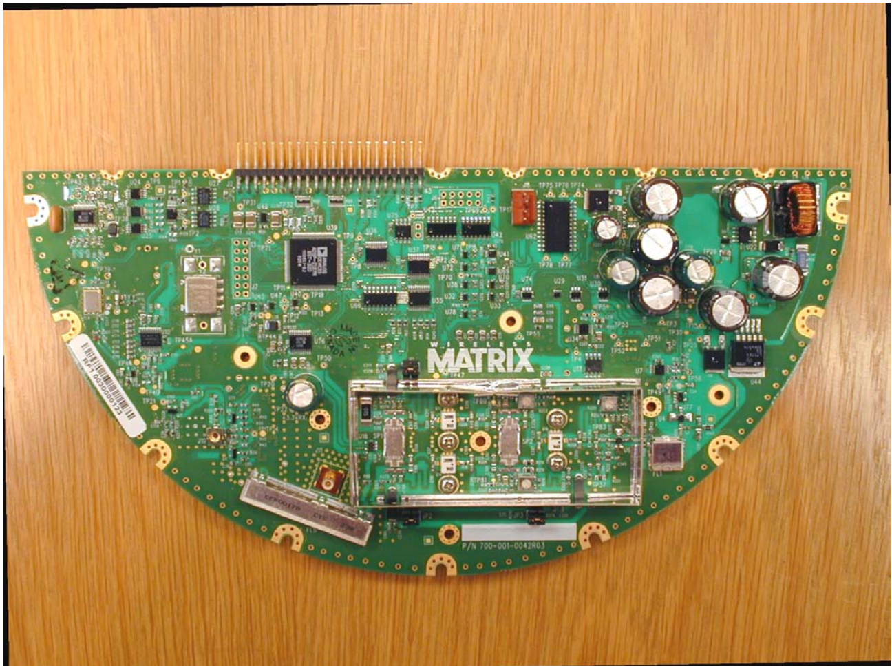
RF1 Board without shield Top view
