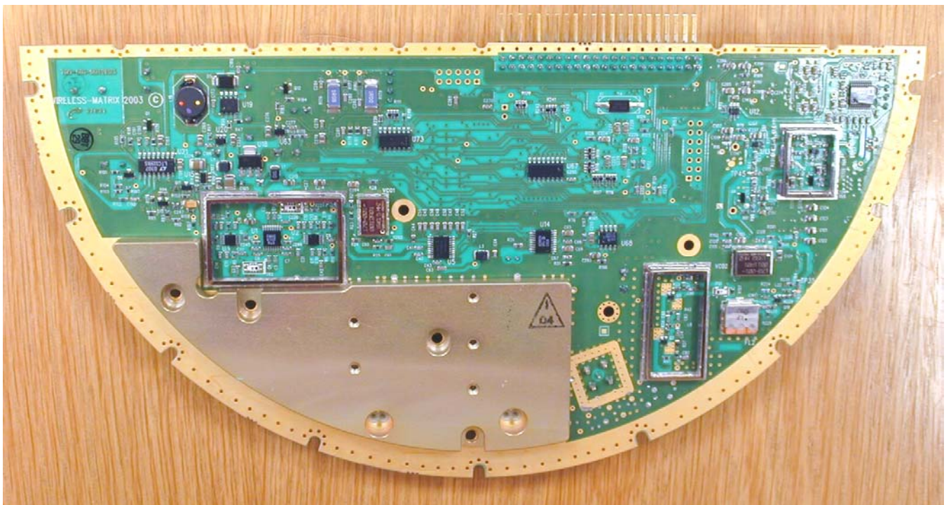
RF1 Board with shield Bottom view
