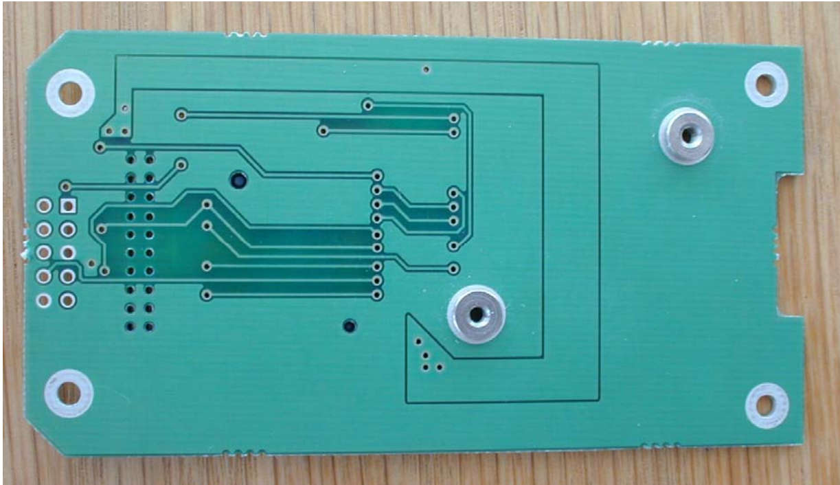
GSM Module carrier board Bottom view
