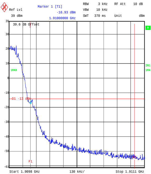
Title: Flextronic EUT: G32a FCC Part 24. Radiated Band Edge Comment A: 48122JD03 Operating in PCS 1900, Top Channel, GPRS Mode. Date: 10.JUL.2006 12:00:56
