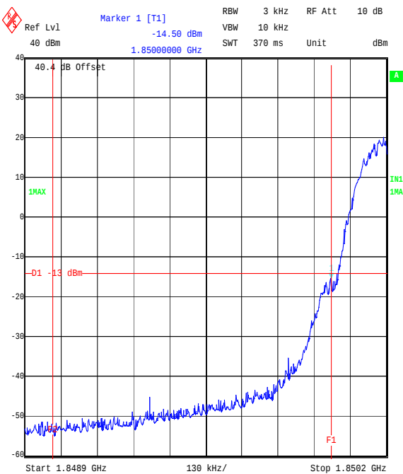
Title: Flextronic EUT: G32a FCC Part 24. Radiated Band Edge Comment A: 48122JD03 Operating in PCS 1900, Bottom Channel, GPRS Mode. Date: 10.JUL.2006 11:57:00
