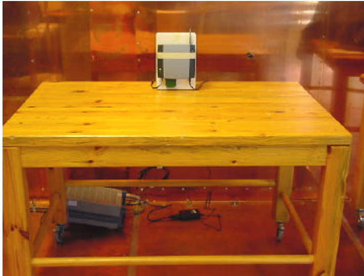
Test set-up Conducted disturbance voltage 0,15 - 30 MHz
