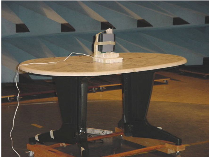
Test set-up 30 – 1000 MHz
