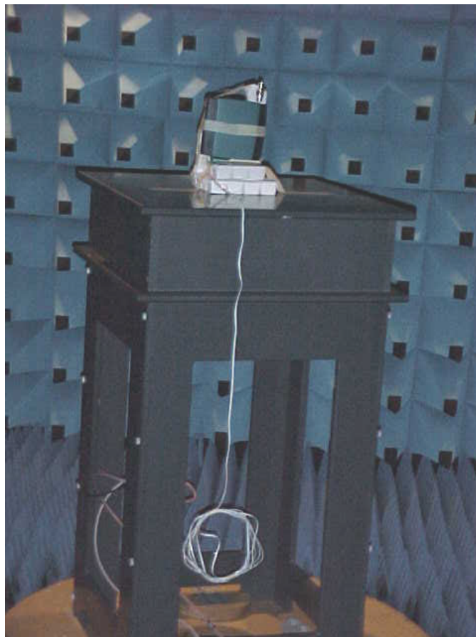
Test set-up 1 – 26 GHz
