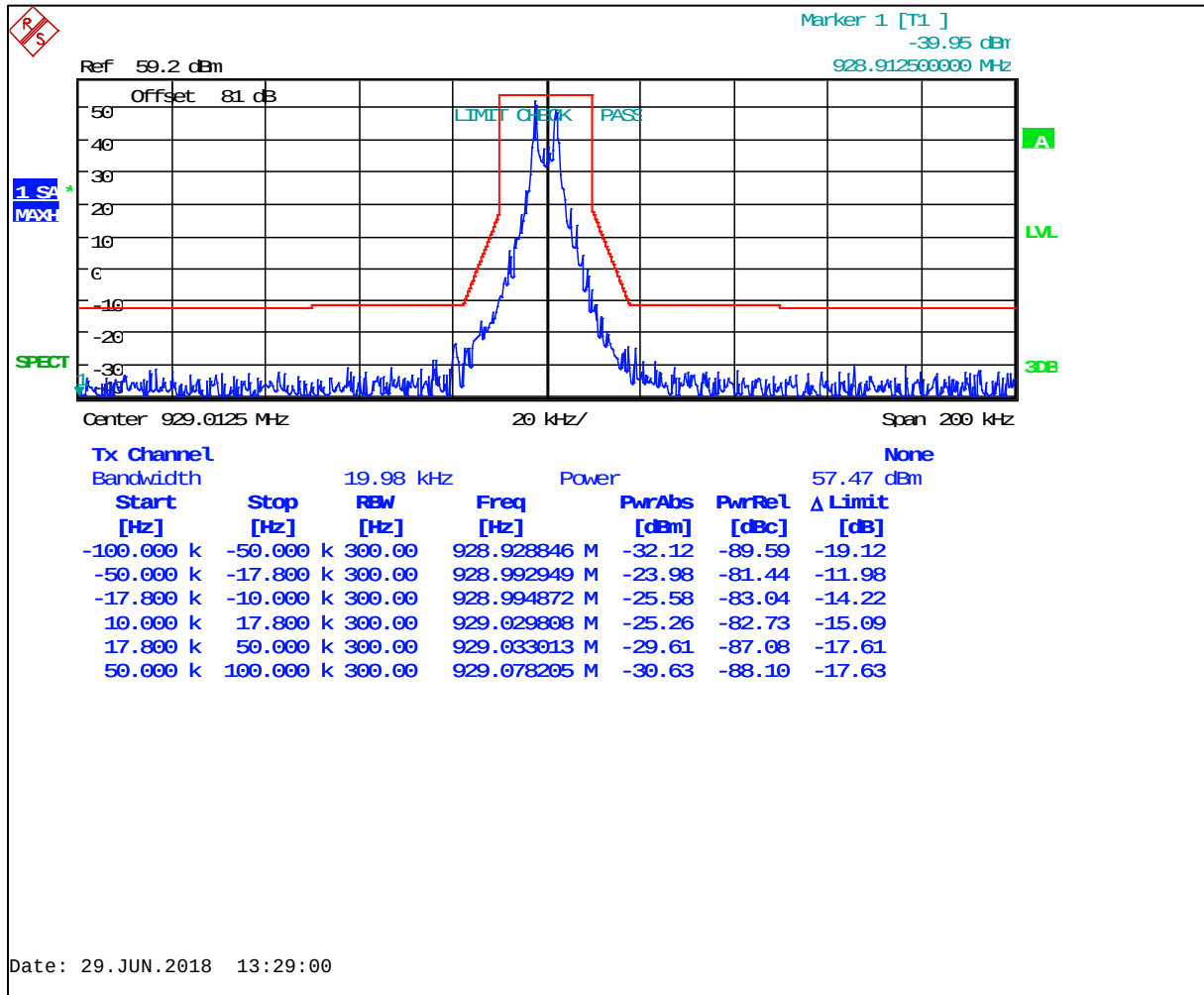
Plot 8-2: Emission Masks - 929.0125 MHz, 12.5 kHz Bandwidth, High Power; POCSAG 1200 PRBS- Mask G
