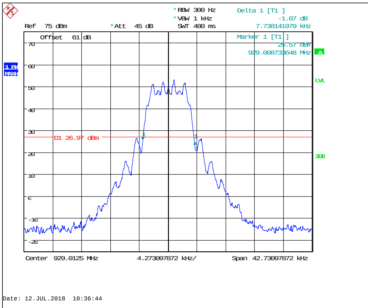
Plot 8-41: 26 dB Bandwidth – 929.0125 MHz, 12.5 kHz Bandwidth, High Power; FLEX-4 3200 PRBS
