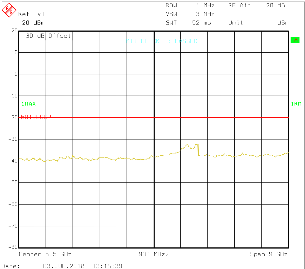
Plot 5-12: Conducted Antenna Spurious Emissions –929.0125 MHz; 1-10 GHz; 12.5 kHz BW; 20W
