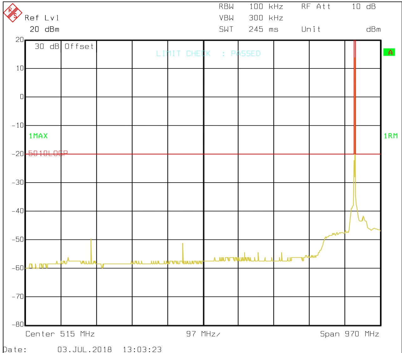
Plot 5-3: Conducted Antenna Spurious Emissions – 929.0125 MHz; 30 MHz–1 GHz; 12.5 kHz BW; 250W
