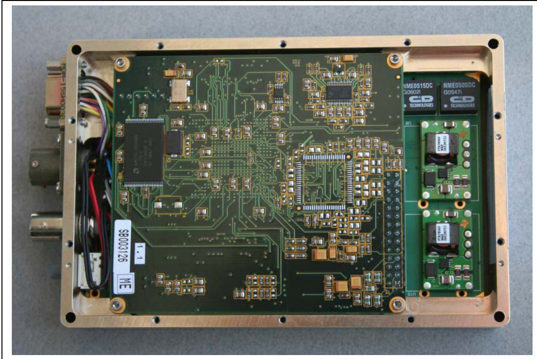
Fig 9. DT-200S Interior Bottom
