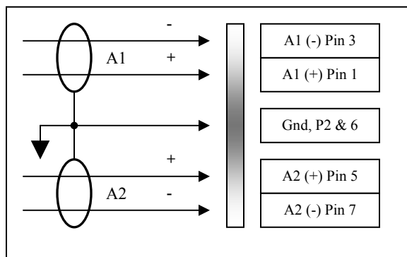
Balanced Audio Input Wiring
