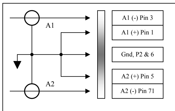
Unbalanced Audio Input Wiring
